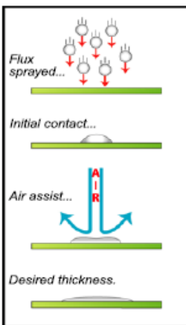
Figure 2: Coaxial air assist spreads the flux and helps achieve final thicknesses as thin as 5\mu .
